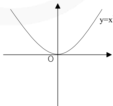
Even function (Symmetric about y-axis)
